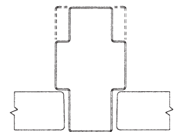
Welded or Removable Mullion Between Doors
