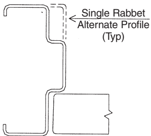
Single Rabbet Alternate Profile (Typ) Door Mounted Lock Strike Jamb, Hinge Jamb Head
