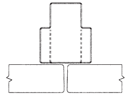
Welded or Removable Mullion Behind Doors
